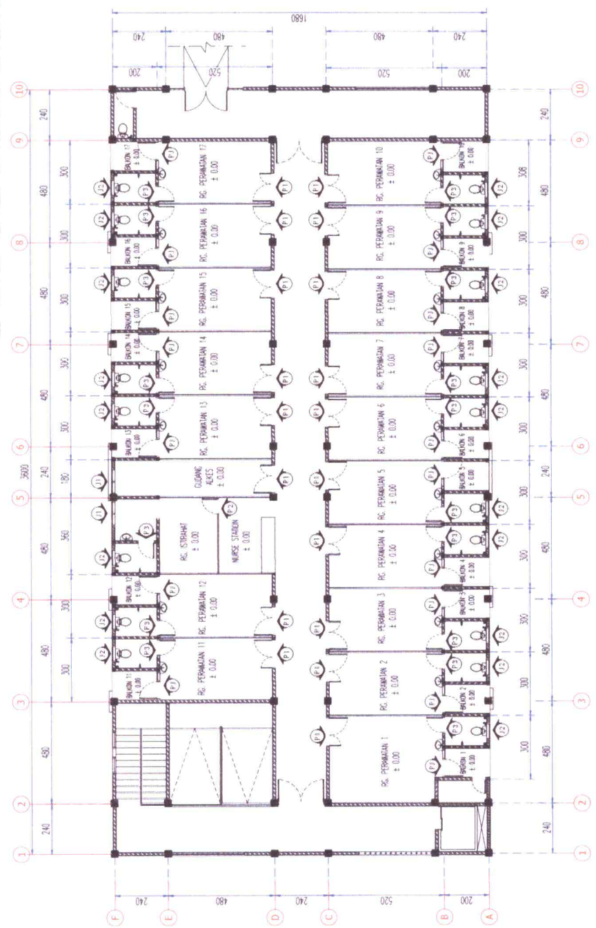
DENAH KUSEN Skala 1 : 150
